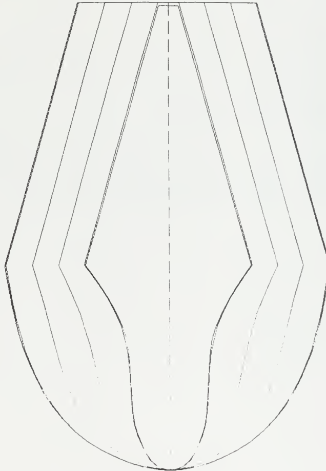
COMP_A.C Body Plan (1 component) Scale = 1:100
